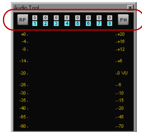
Audio tool. Top, left to right: Reset Peak (RP) button, In/Out toggle buttons, Peak Hold (PH) Menu button. Left display column: Digital scale (fixed). Right display column: Volume unit scale (adjustable).
