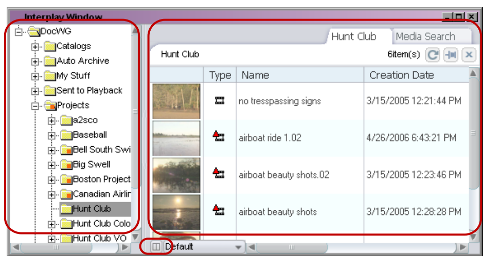
The Interplay Window, showing the Media Directory panel (left), the Research panel (right), and the Layout button (bottom)
