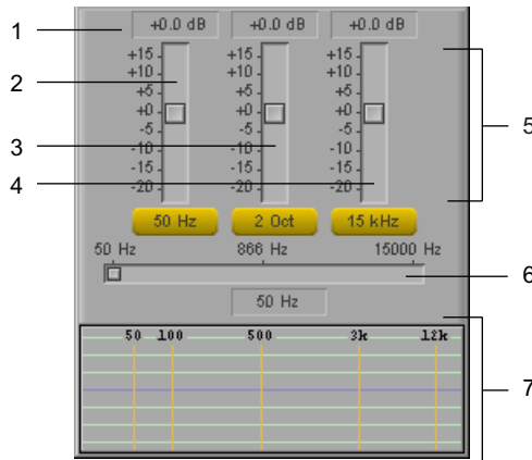
Bottom part of the Audio EQ tool
