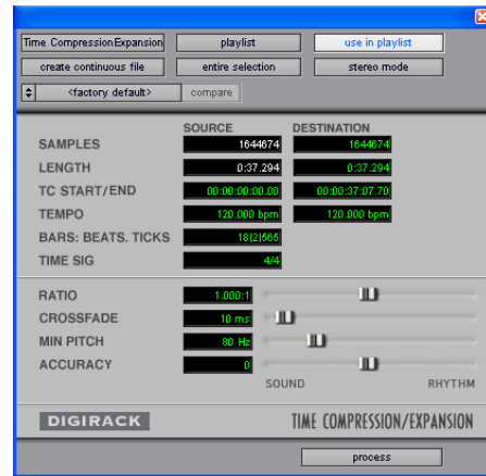
Time Compression/Expansion plug-in
