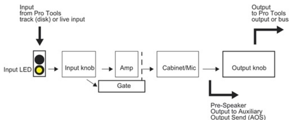
Signal flow through Eleven MK II
