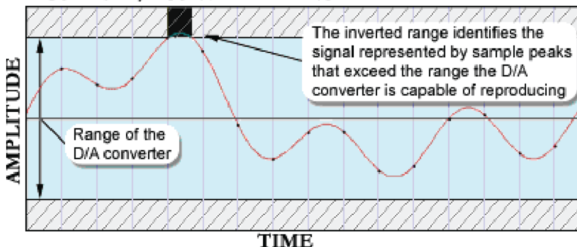
FIGURE 4 - D/A CONVERTER RANGE
