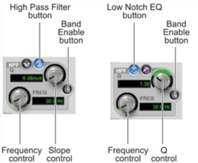
High Pass filter (left) and Low Notch EQ (right)
