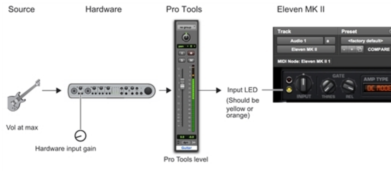
Basic gain stages to calibrate live guitar input for Eleven MK II
