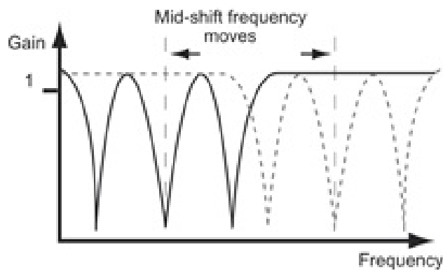
Sweep adjusts the center frequency point
