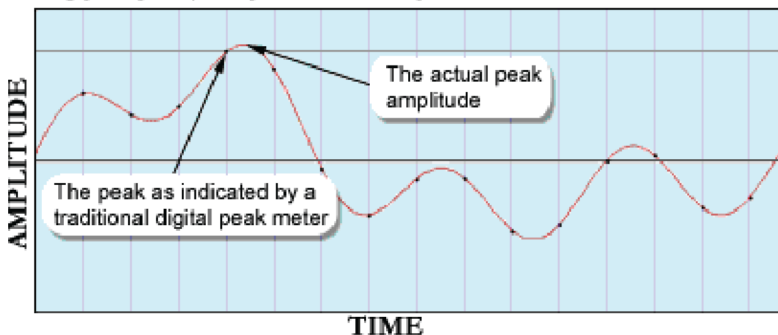
FIGURE 3 - INTERSAMPLE PEAKS
