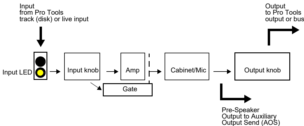
Signal flow through Eleven MK II
