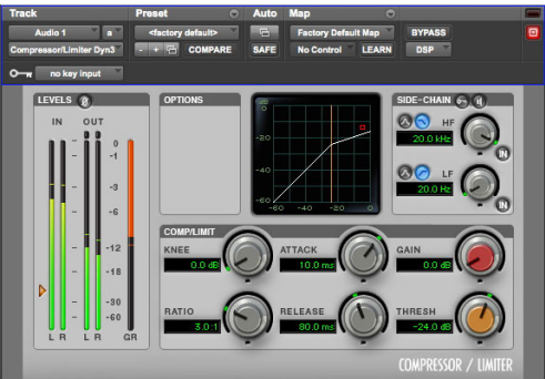
Compressor/Limiter III
