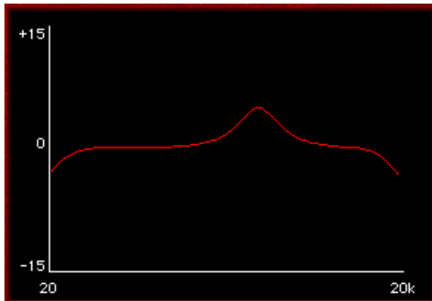
Cartesian Graph
